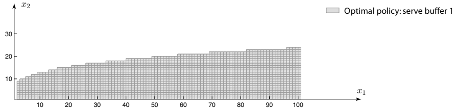
Figure 5: Average cost optimal policy for the tandem queues with c_1 = 1 , c_2 = 3 , \rho_1 = 9/11 , \rho_2 = 9/10 .
