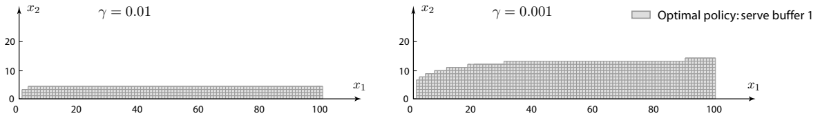
Figure 4: Discounted cost optimal policy for the tandem queues with cost parameters (c_1, c_2) = (1, 3) . The load parameters are \rho_1 = 9/10 , \rho_2 = 9/11 , and the linear cost defined by c_1 = 1 , c_2 = 3 . On the left \gamma = 0.01 and on the right \gamma = 0.001 .
