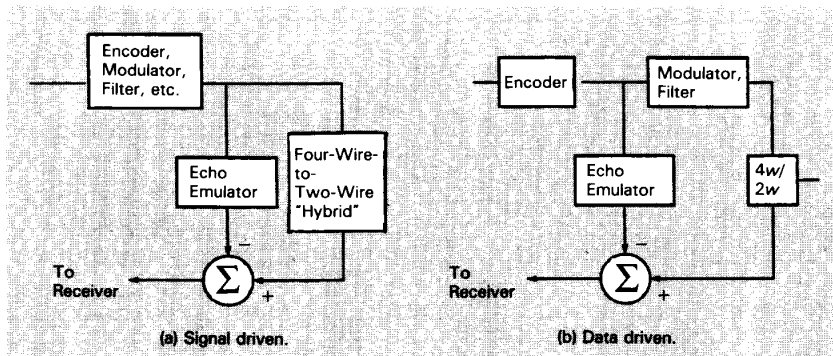
Fig. 8. Echo cancelers.
