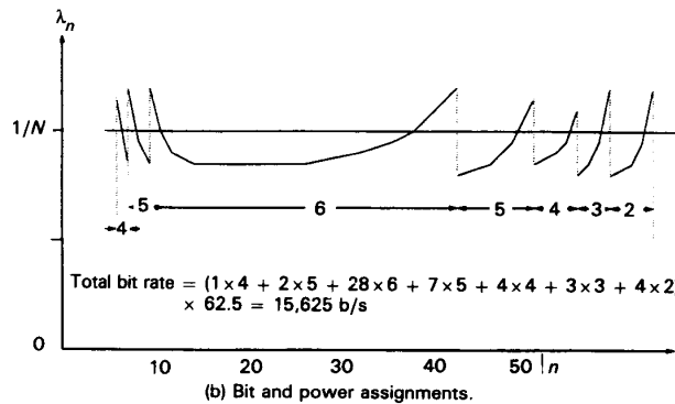
Fig. 3. Adaptive loading for a badly distorted GSTN channel.
