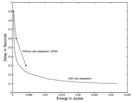
Fig. 8. Delay and energy tradeoff, transmission energy only
