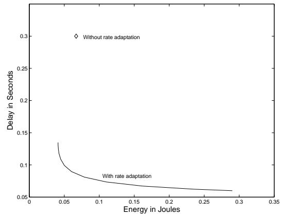
Fig. 9. Delay and energy tradeoff, circuit energy consumption included
