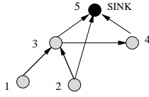
Fig. 7. Scheduling example
